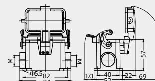
1) : Structure 1 ( M=M25 Using Structure 1)
