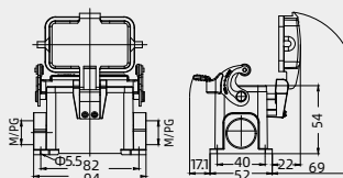
Structure 2: M/PG=M20/PG16 Using Structure 2
